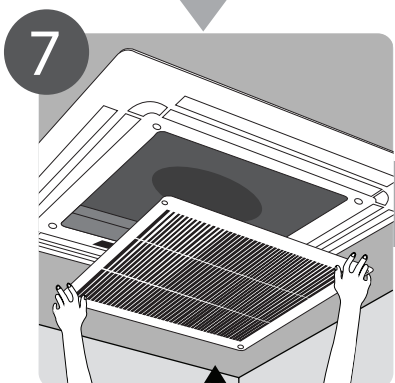
7 Install the front panel
