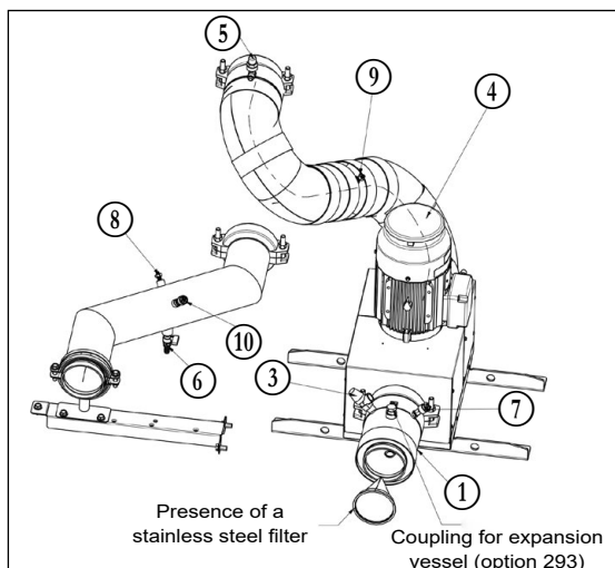
Example: Single-pump
