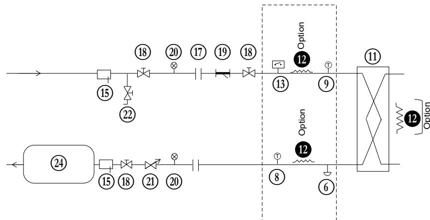
Typical hydraulic circuit diagram without hydraulic module
