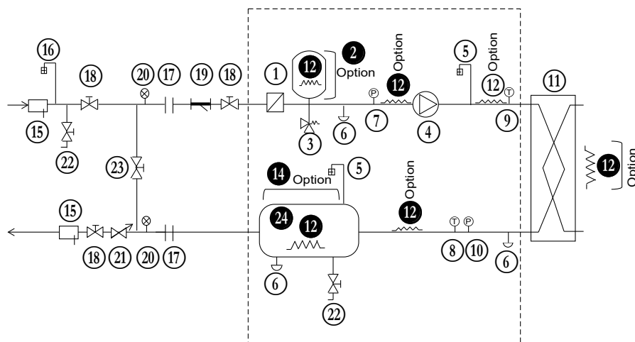
Typical hydraulic circuit diagram with hydraulic module
