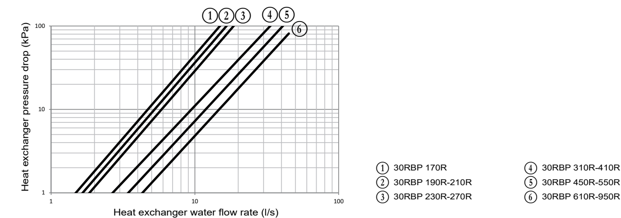
Total recovery (pressure drop curves for the plate heat exchangers)
