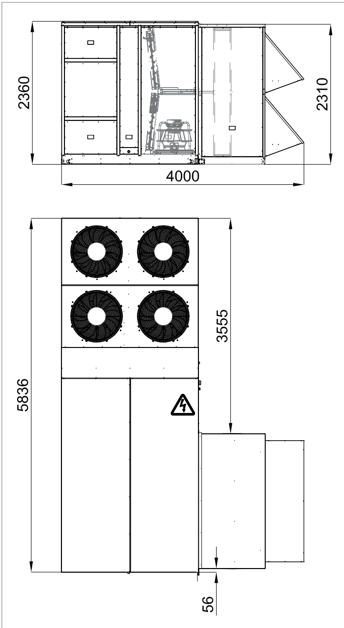
Fig. 16.10 -ERM 29.6 E / S and 50/48 UC-(V)UP-(V) 190-220
