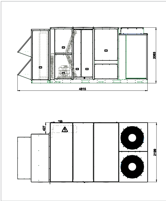
Fig. 16.4 - ERM 11.4 E / S; ERM 13.4 E / S; ERM 174 E / S and 50/48 UC-(V) / UP-(V) 065,075,090,105 Rooftop unit installation
