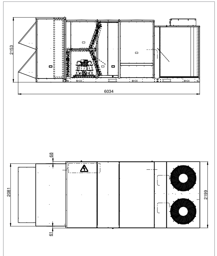
Fig. 16.6 -ERM 23.5 E / S and 50/48 UC-(V)/UP-(V) 125, Rooftop unit installation
