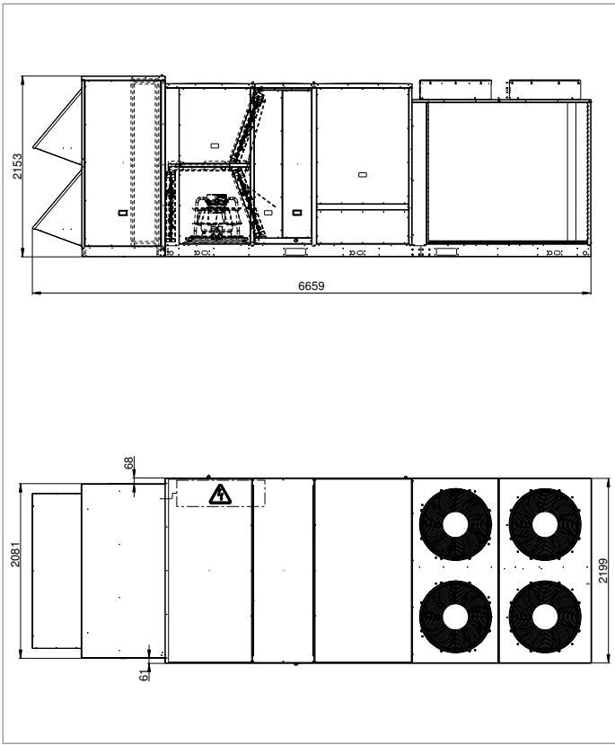
Fig. 16.8 -ERM 23.5 E / S and 50/48 UC-(V)/UP-(V) 160 Rooftop unit installation
