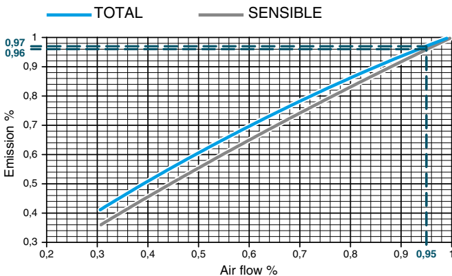
Diagram 1 - Cooling emissions
