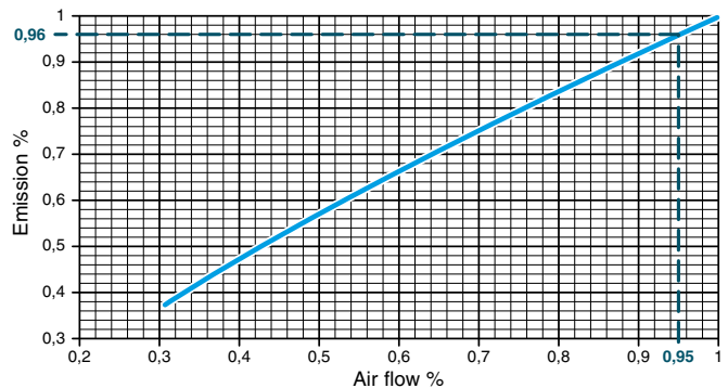
Diagram 2 - Heating emission
