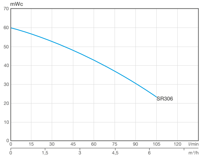
Pump Flow (Q) - Pressure (H) Table
