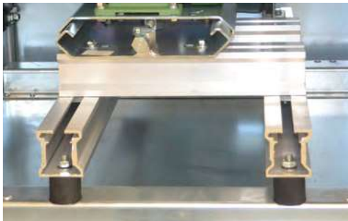
Rubber anti vibration mounts
