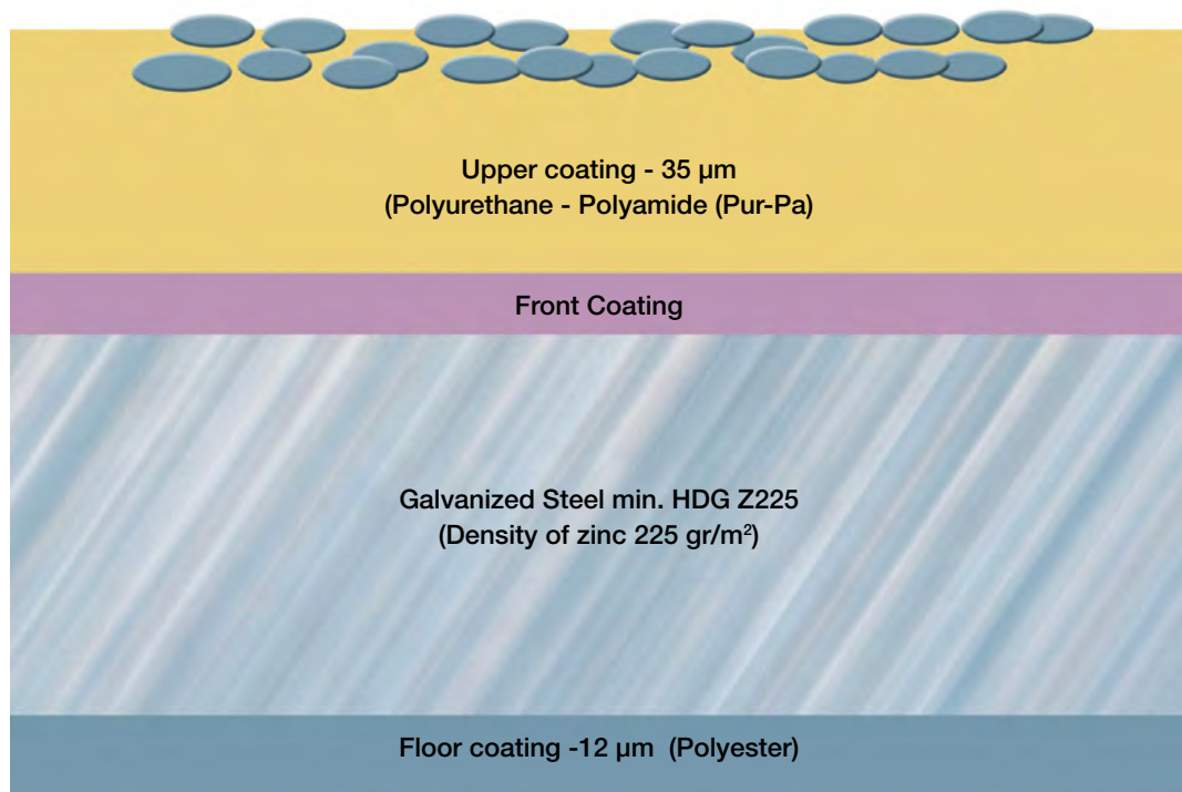
Panel coating
