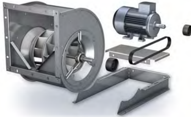
Belt-driven fans
